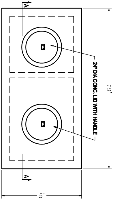
PLAN VIEW
